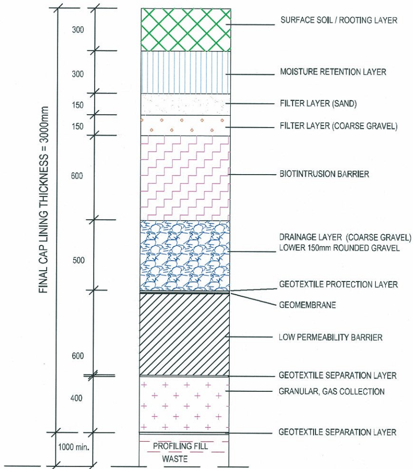
SECTION THROUGH FINAL CAP
